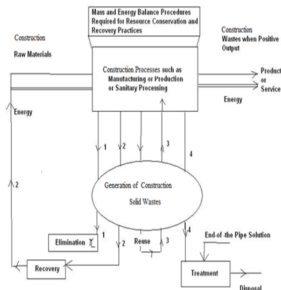
Figure - 9 : Schematic Representation of Constructional Process or Activity Showing Sustainable Construction Waste Management
